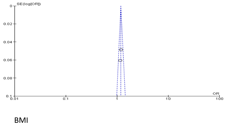
Fig. 3 Funnel plot for risk factors of HG among pregnant women
